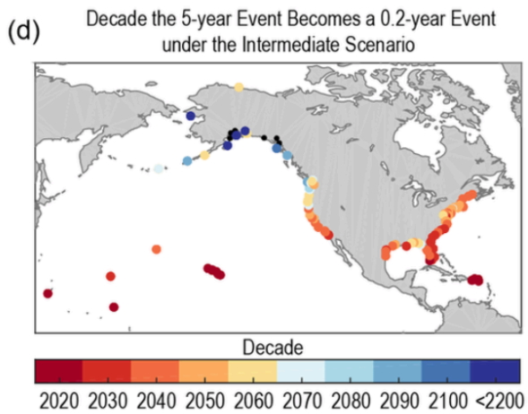
Figure 4. NOAA model for high tide flooding; decade the 5-year king tide becomes the 5 times per year king tide (2020).
