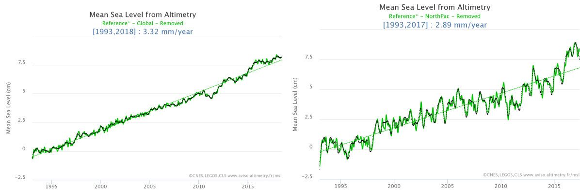
Figure 1. Left Global mean sea level. Right North Pacific mean sea level.
